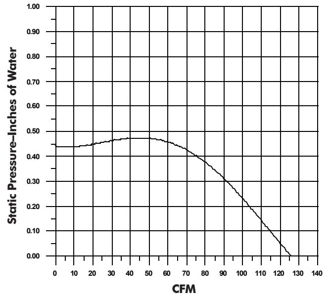
NuVent Product Performance Model NXMS110FL
